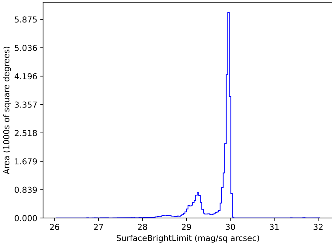
noroll_mjdp180_v3.4_10yrs i: SurfaceBrightLimit
