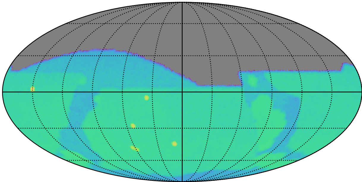
noroll_mjdp180_v3.4_10yrs g: SurfaceBrightLimit
