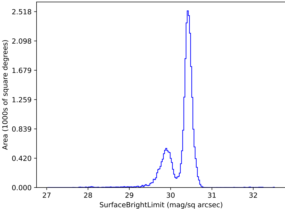
noroll_mjdp180_v3.4_10yrs g: SurfaceBrightLimit
