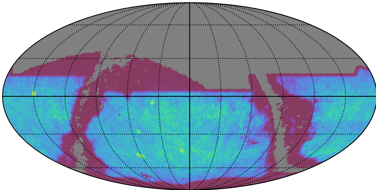
noroll_mjdp180_v3.4_10yrs : SNSLMetric
