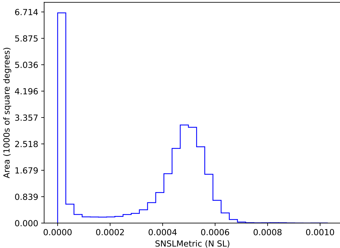
noroll_mjdp180_v3.4_10yrs : SNSLMetric
