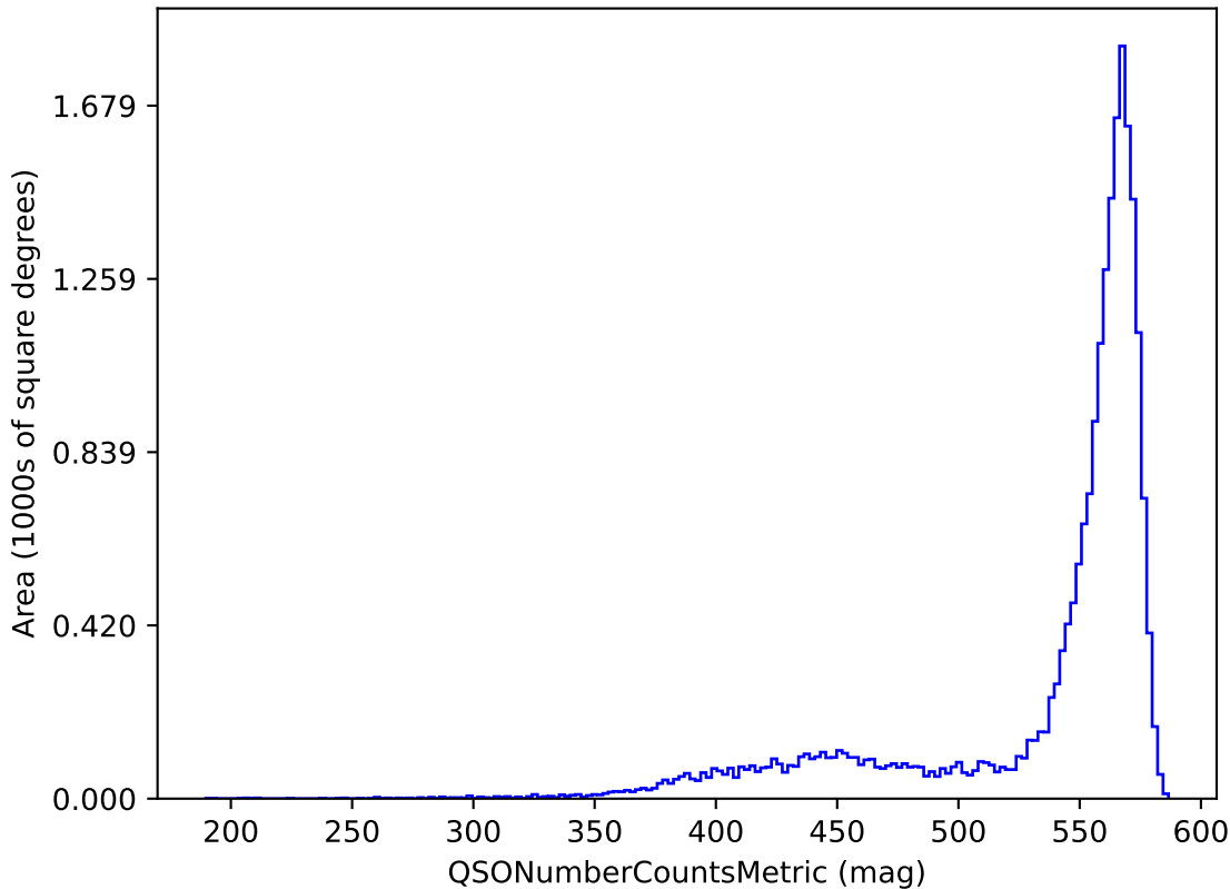
noroll_mjdp180_v3.4_10yrs y band and non-DD: QSONumberCountsMetric
