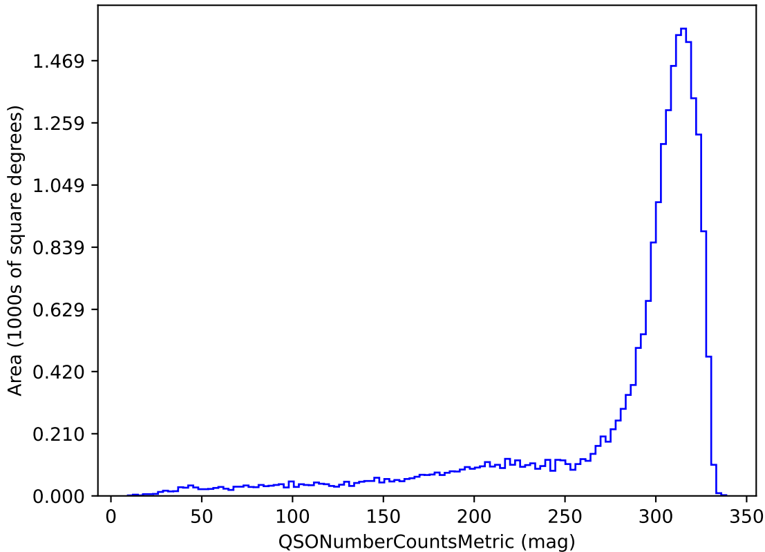
noroll_mjdp180_v3.4_10yrs u band and non-DD: QSONumberCountsMetric
