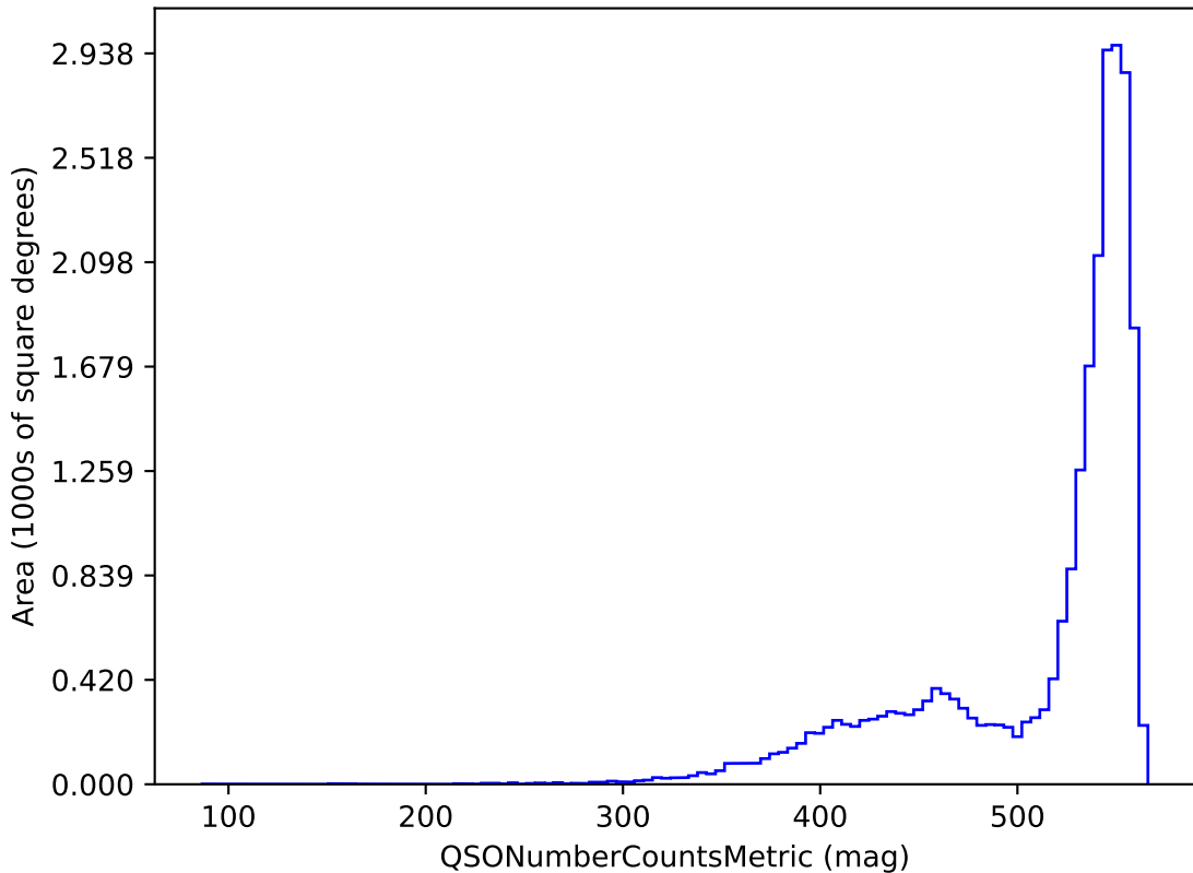
noroll_mjdp180_v3.4_10yrs i band and non-DD: QSONumberCountsMetric
