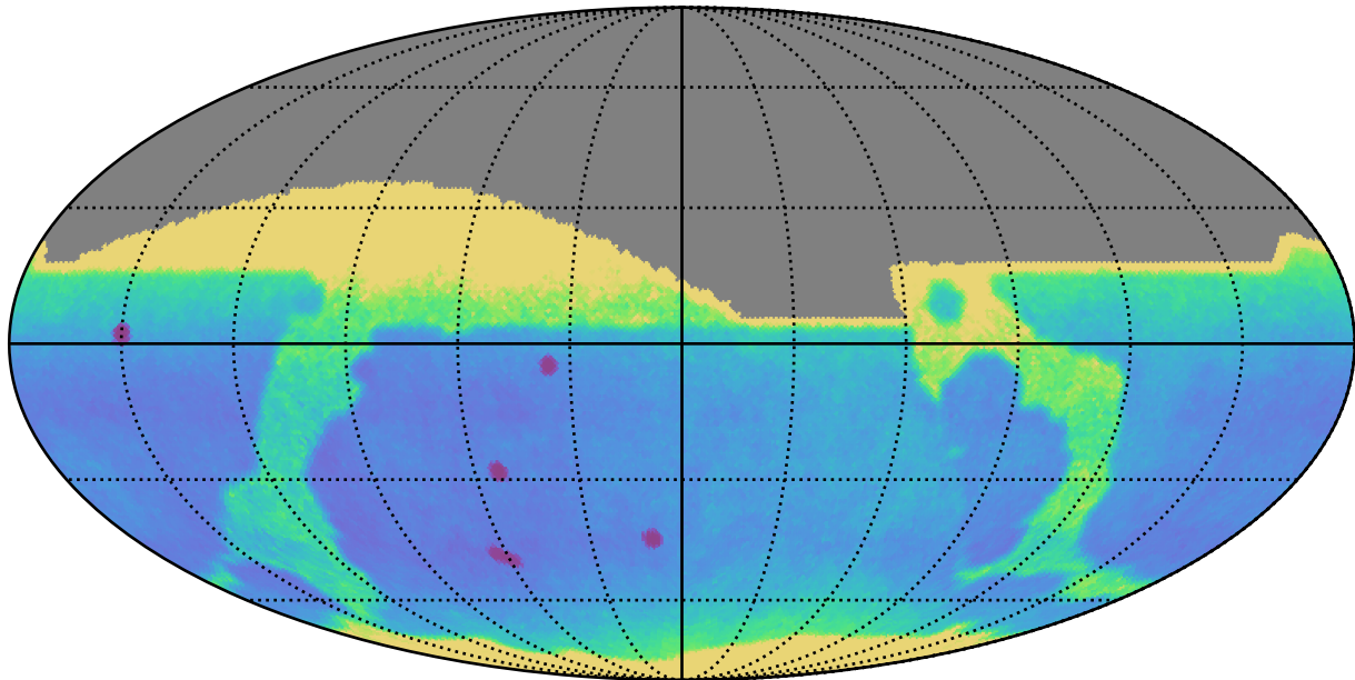
noroll_mjdp180_v3.4_10yrs : Proper Motion Uncert @ 24.0
