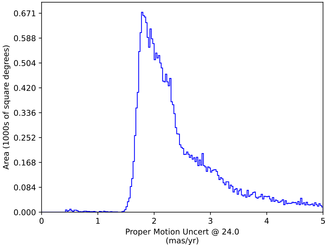
noroll_mjdp180_v3.4_10yrs : Proper Motion Uncert @ 24.0
