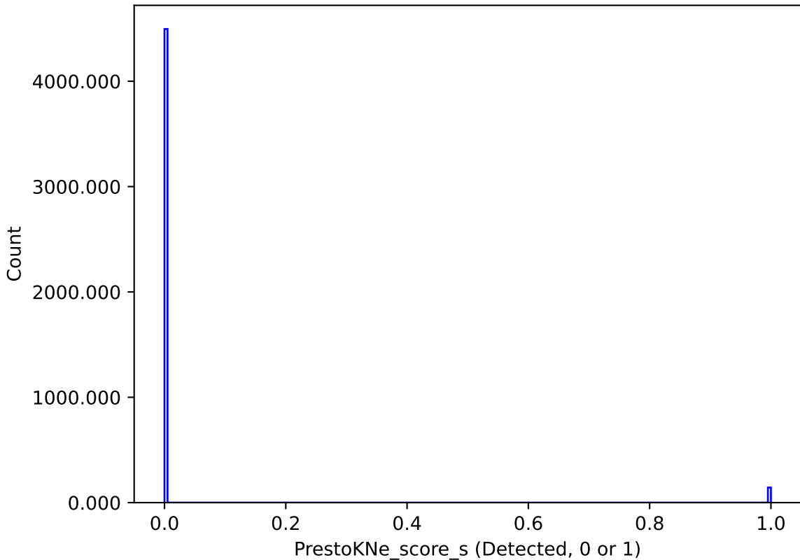
noroll_mjdp180_v3.4_10yrs : PrestoKNe_score_s
