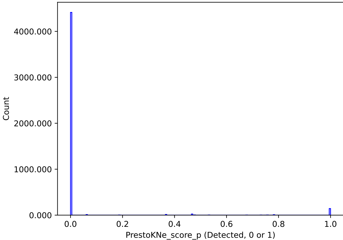
noroll_mjdp180_v3.4_10yrs : PrestoKNe_score_p
