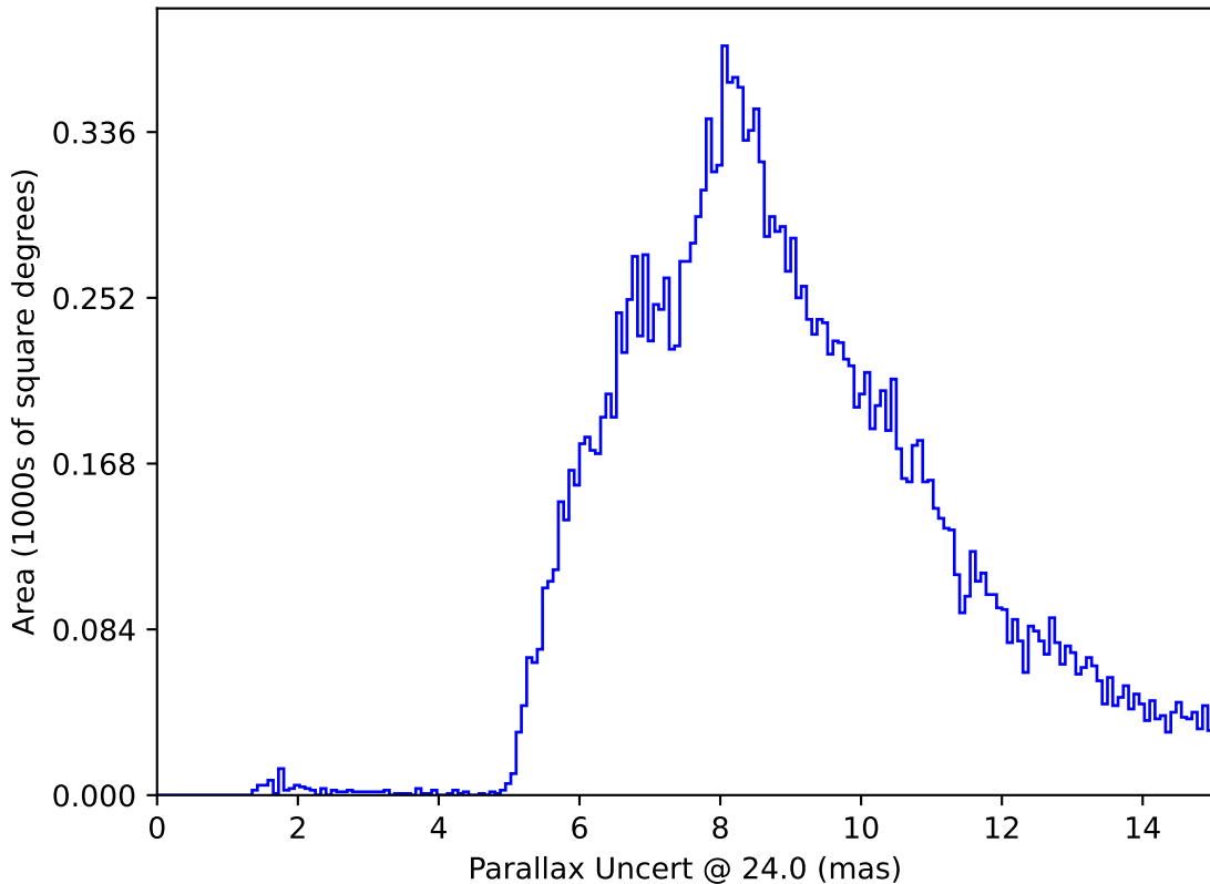
noroll_mjdp180_v3.4_10yrs : Parallax Uncert @ 24.0
