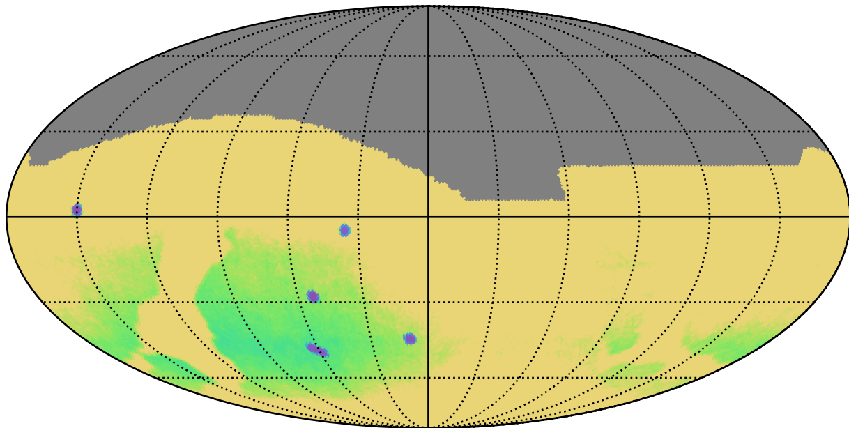
noroll_mjdp180_v3.4_10yrs : Parallax Uncert @ 22.4
