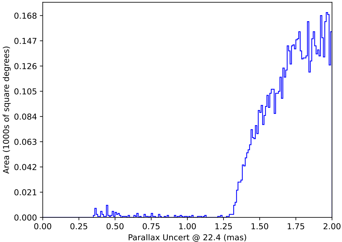
noroll_mjdp180_v3.4_10yrs : Parallax Uncert @ 22.4
