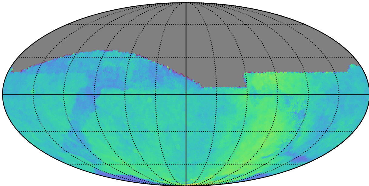
noroll_mjdp180_v3.4_10yrs : Parallax Coverage @ 24.0
