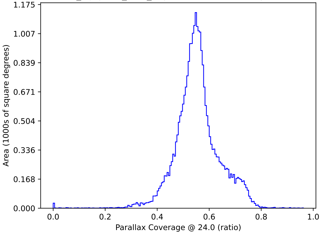
noroll_mjdp180_v3.4_10yrs : Parallax Coverage @ 24.0
