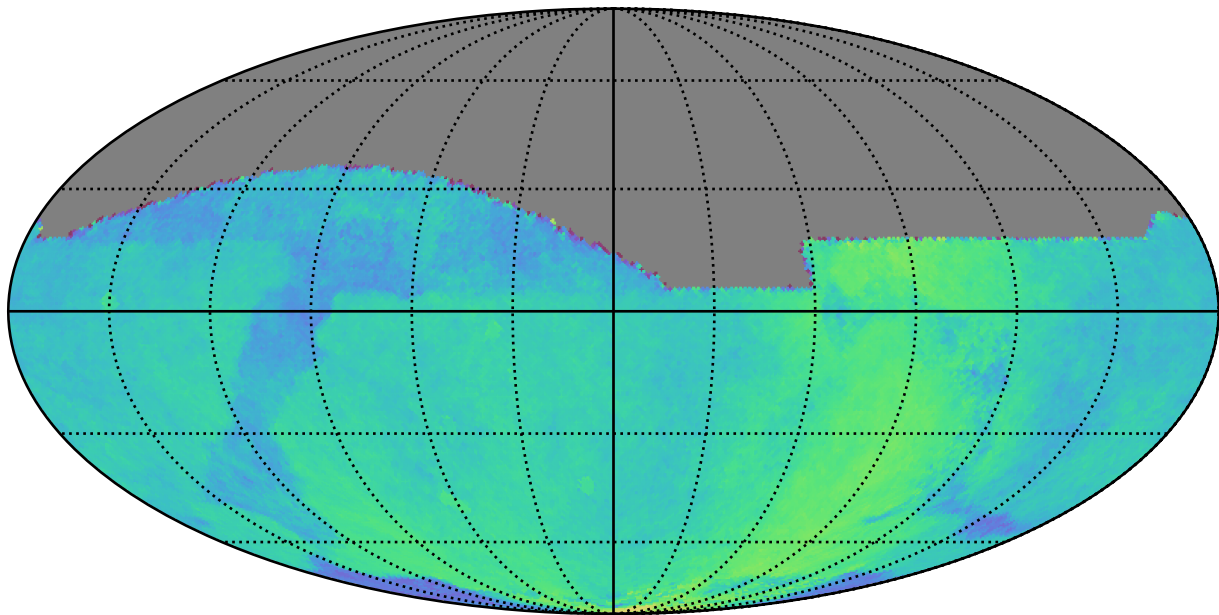
noroll_mjdp180_v3.4_10yrs : Parallax Coverage @ 22.4
