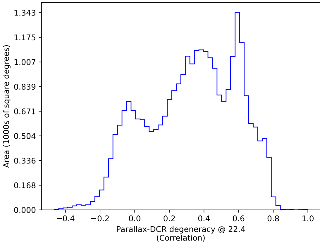
noroll_mjdp180_v3.4_10yrs : Parallax-DCR degeneracy @ 22.4
