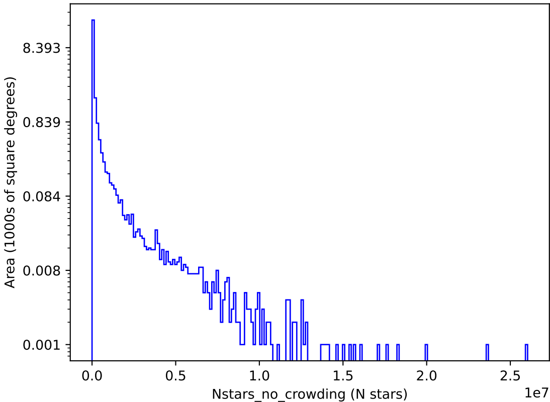
noroll_mjdp180_v3.4_10yrs y: Nstars_no_crowding
