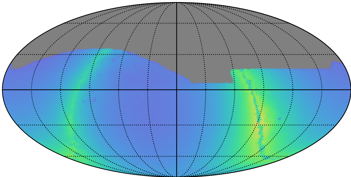
noroll_mjdp180_v3.4_10yrs r: Nstars_no_crowding
