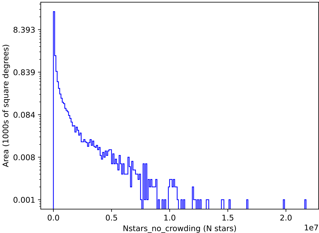
noroll_mjdp180_v3.4_10yrs r: Nstars_no_crowding
