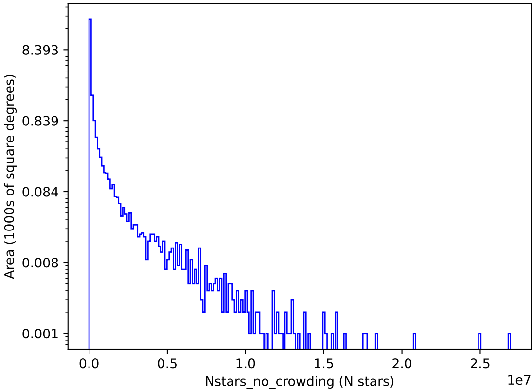
noroll_mjdp180_v3.4_10yrs i: Nstars_no_crowding
