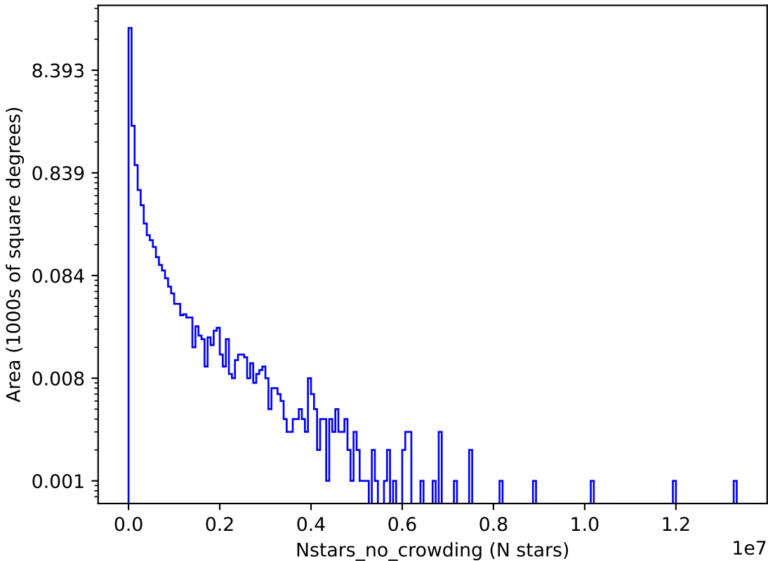
noroll_mjdp180_v3.4_10yrs g: Nstars_no_crowding
