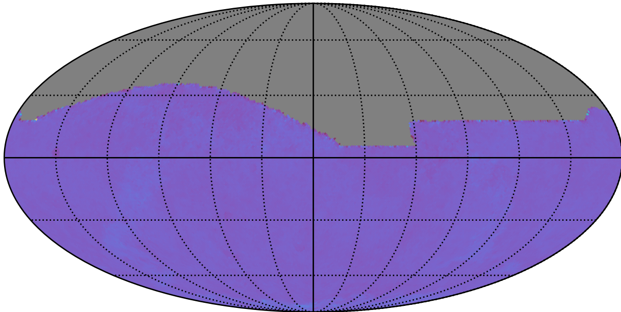
noroll_mjdp180_v3.4_10yrs : Normalized Proper Motion Uncert @ 24.0
