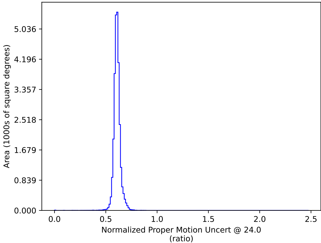
noroll_mjdp180_v3.4_10yrs : Normalized Proper Motion Uncert @ 24.0
