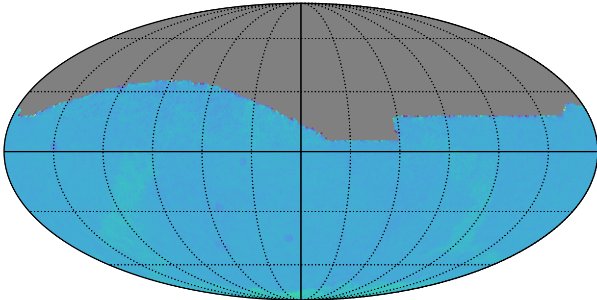
noroll_mjdp180_v3.4_10yrs : Normalized Proper Motion Uncert @ 20.5
