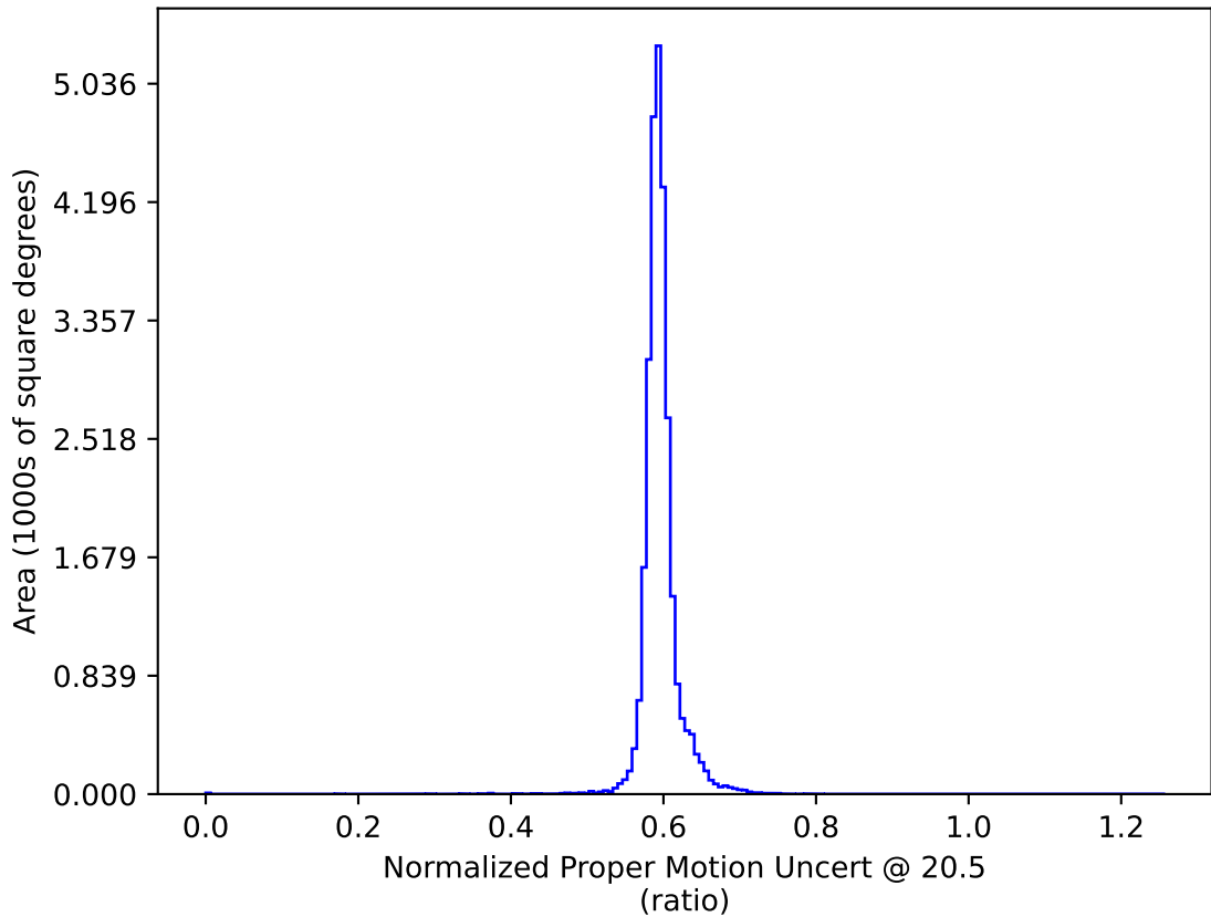
noroll_mjdp180_v3.4_10yrs : Normalized Proper Motion Uncert @ 20.5
