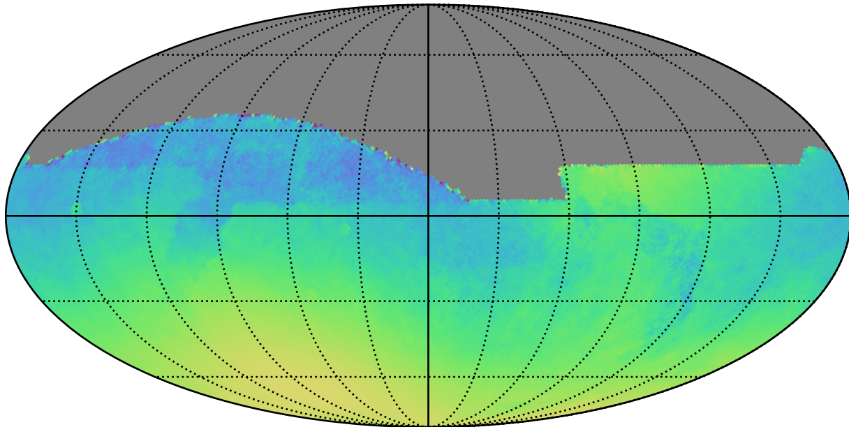
noroll_mjdp180_v3.4_10yrs : Normalized Parallax Uncert @ 24.0
