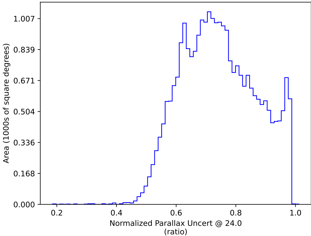
noroll_mjdp180_v3.4_10yrs : Normalized Parallax Uncert @ 24.0
