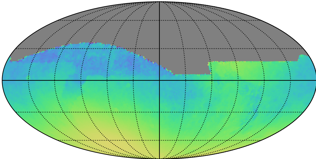
noroll_mjdp180_v3.4_10yrs : Normalized Parallax Uncert @ 22.4
