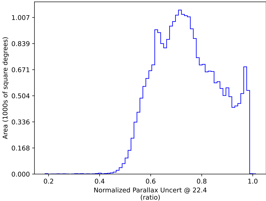
noroll_mjdp180_v3.4_10yrs : Normalized Parallax Uncert @ 22.4
