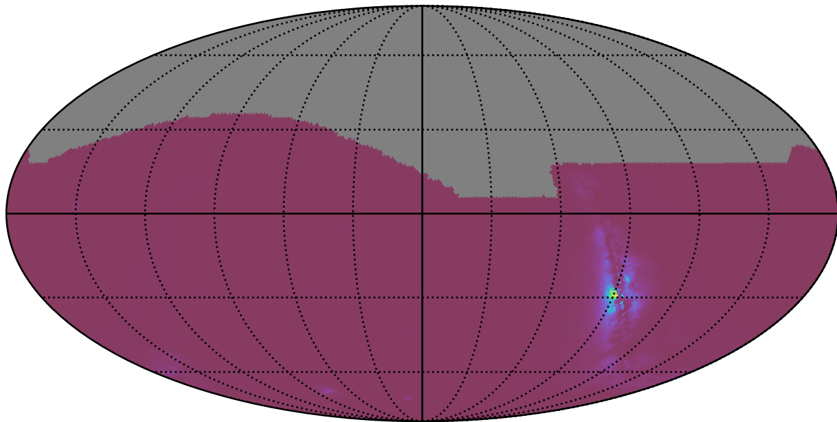
noroll_mjdp180_v3.4_10yrs : NlcPoints
