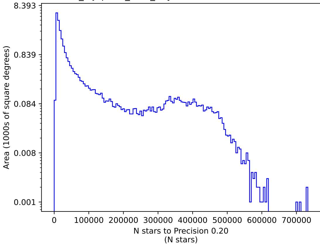
noroll_mjdp180_v3.4_10yrs z: N stars to Precision 0.20
