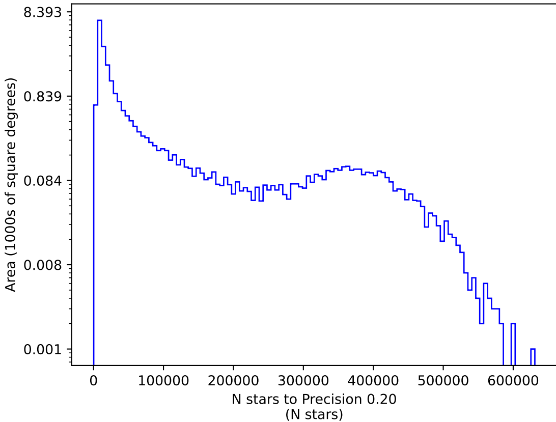
noroll_mjdp180_v3.4_10yrs y: N stars to Precision 0.20
