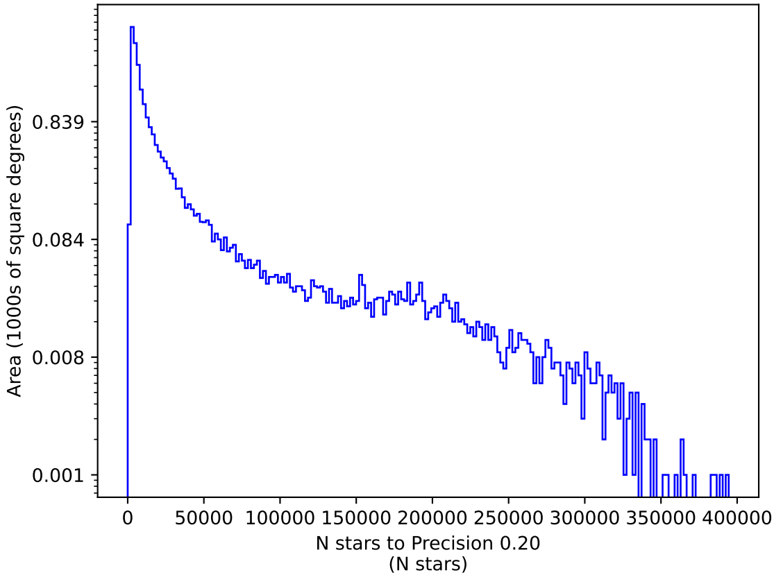
noroll_mjdp180_v3.4_10yrs u: N stars to Precision 0.20
