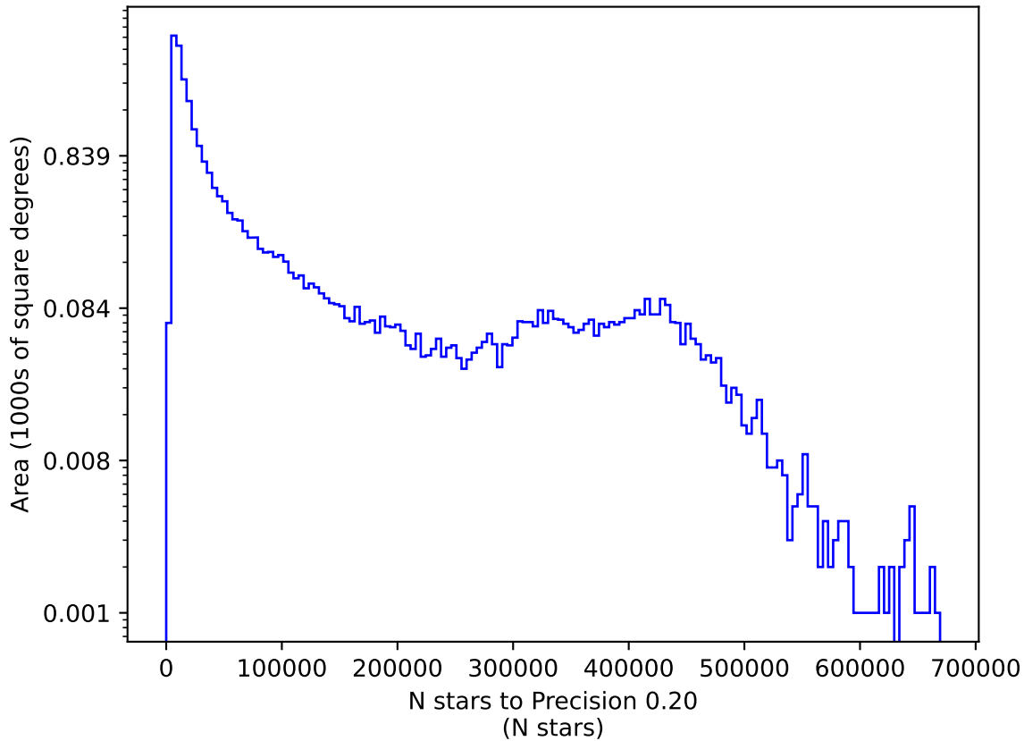
noroll_mjdp180_v3.4_10yrs r: N stars to Precision 0.20
