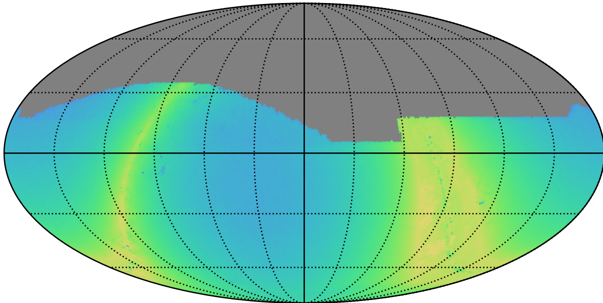
noroll_mjdp180_v3.4_10yrs i: N stars to Precision 0.20
