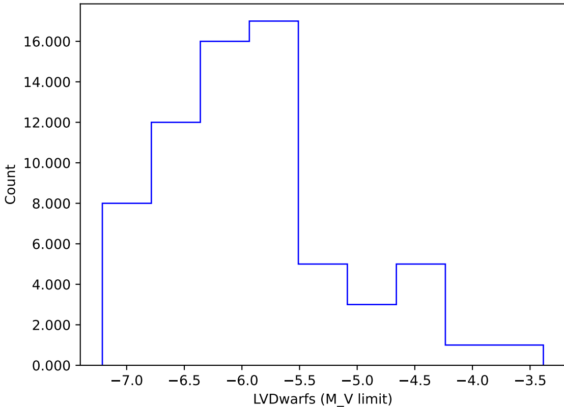
noroll_mjdp180_v3.4_10yrs gi: LVDwarfs
