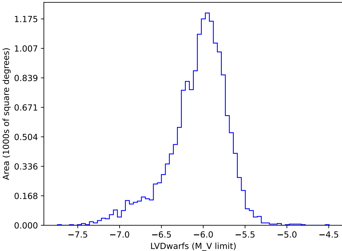
noroll_mjdp180_v3.4_10yrs gi: LVDwarfs
