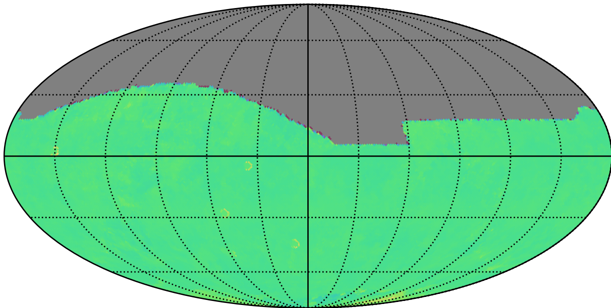
noroll_mjdp180_v3.4_10yrs r: Kuiper rotTelPos
