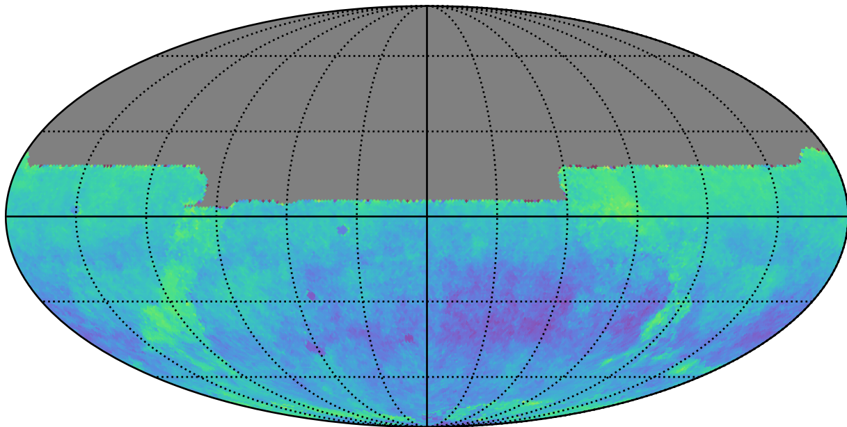
noroll_mjdp180_v3.4_10yrs y: Kuiper rotSkyPos
