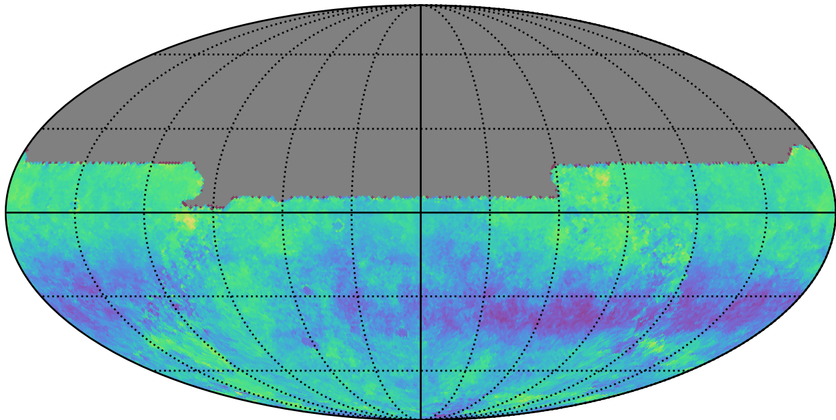
noroll_mjdp180_v3.4_10yrs u: Kuiper rotSkyPos
