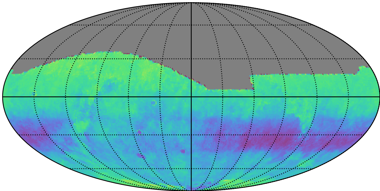
noroll_mjdp180_v3.4_10yrs r: Kuiper rotSkyPos
