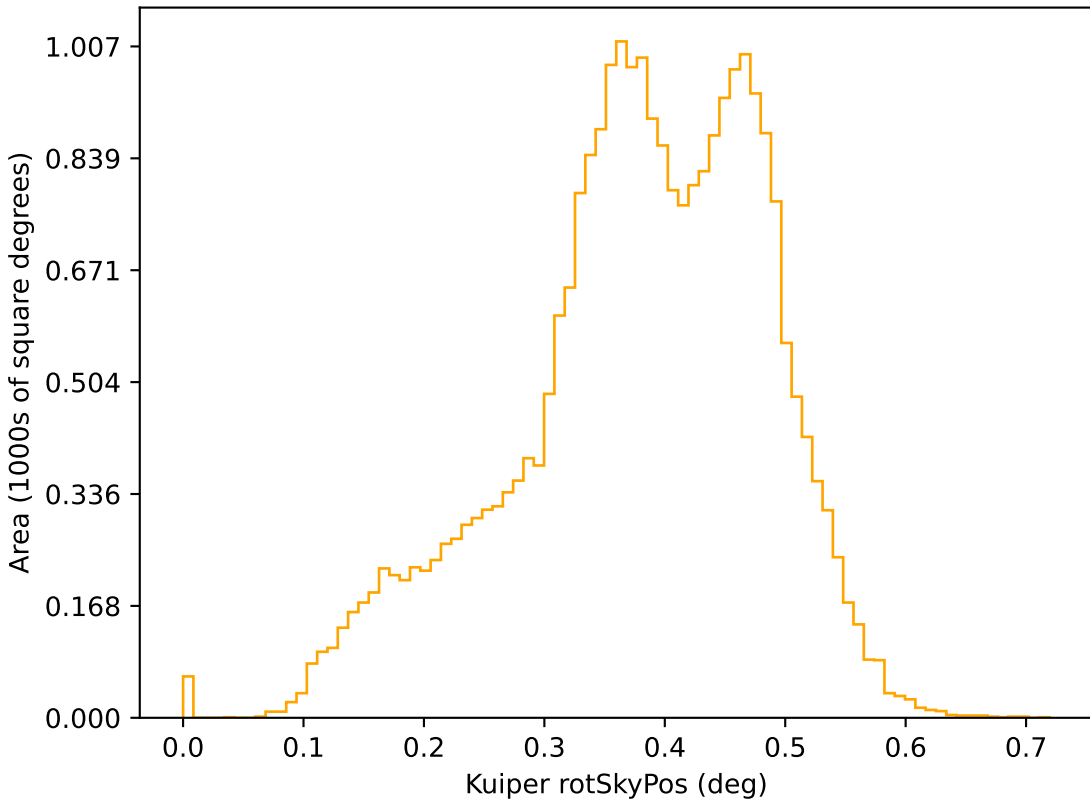
noroll_mjdp180_v3.4_10yrs r: Kuiper rotSkyPos
