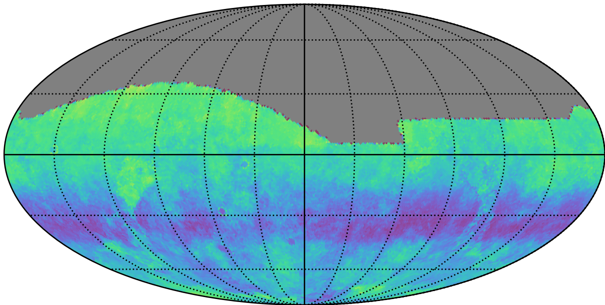
noroll_mjdp180_v3.4_10yrs g: Kuiper rotSkyPos
