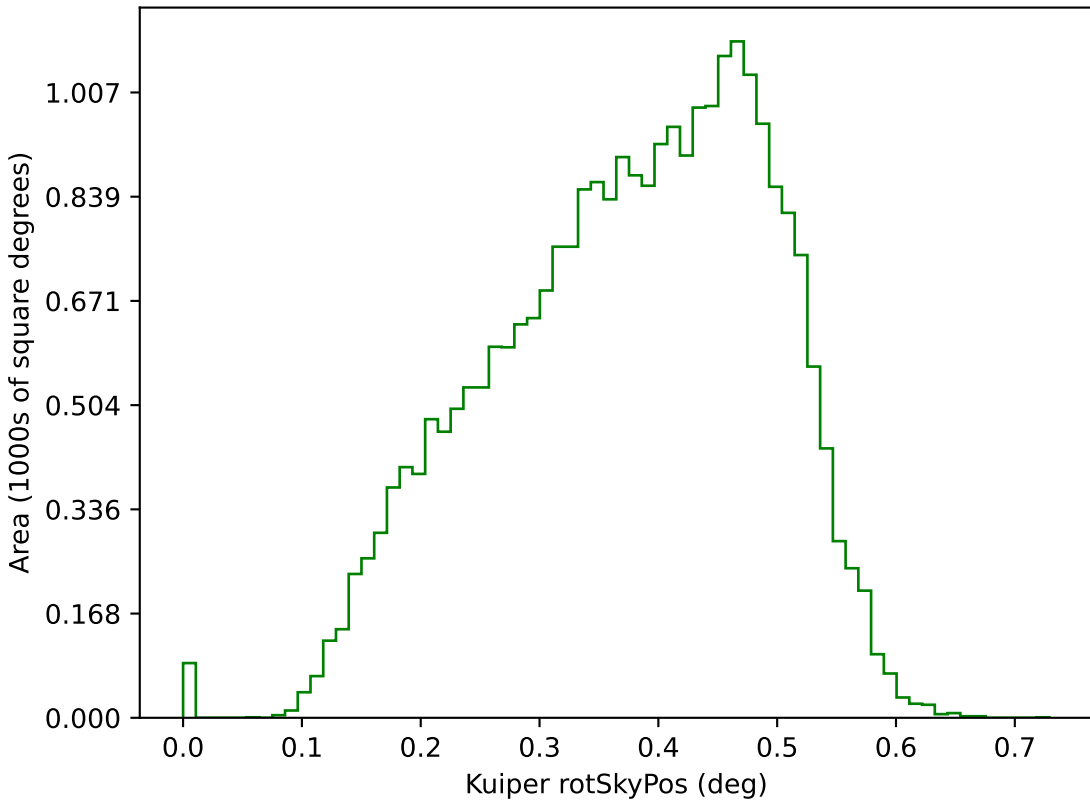
noroll_mjdp180_v3.4_10yrs g: Kuiper rotSkyPos
