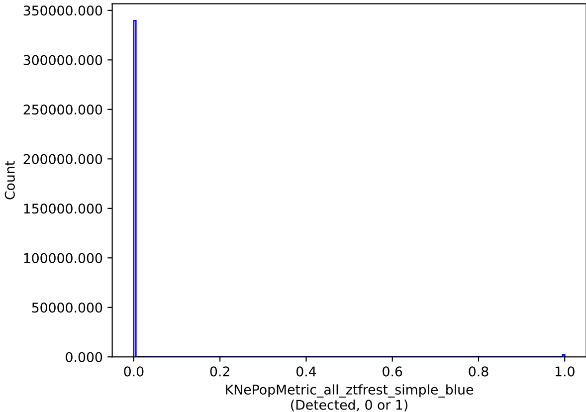
noroll_mjdp180_v3.4_10yrs all models: KNePopMetric_all_ztfrest_simple_blue
