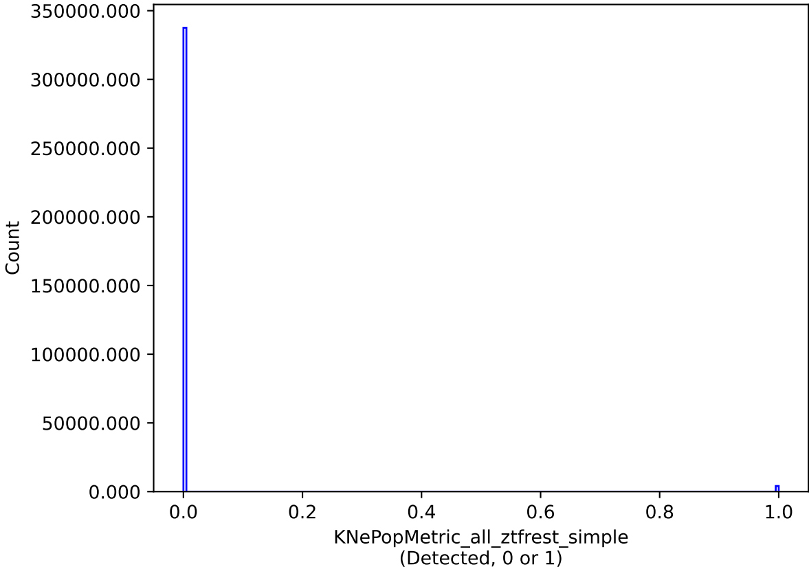
noroll_mjdp180_v3.4_10yrs all models: KNePopMetric_all_ztfrest_simple
