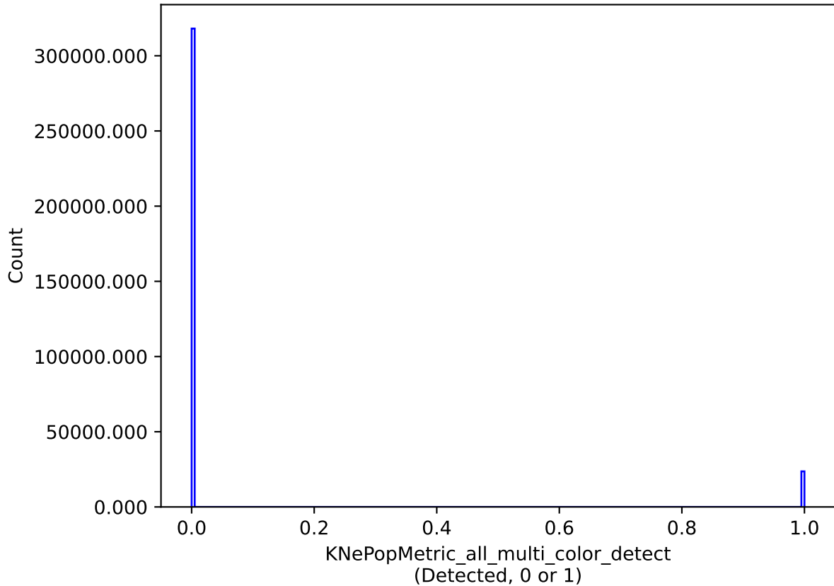
noroll_mjdp180_v3.4_10yrs all models: KNePopMetric_all_multi_color_detect
